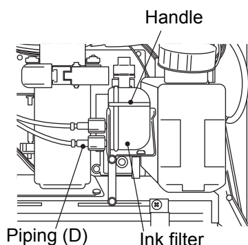
During normal operation/ink disposal
